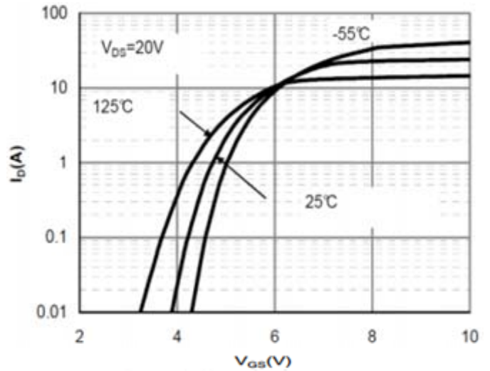
Transfer Characteristics
