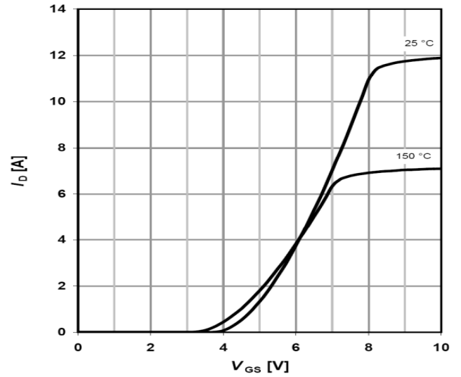
Transfer Characteristic
