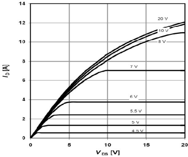
Output Characteristic
