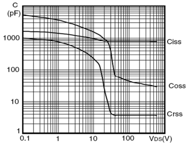
Capacitance
