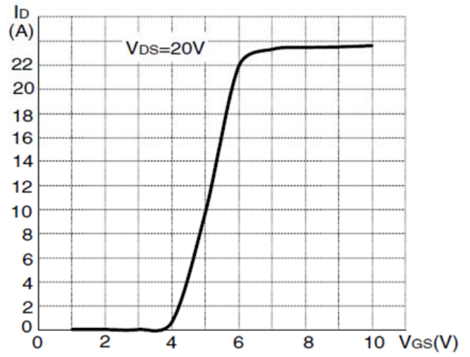
Transfer Characteristic
