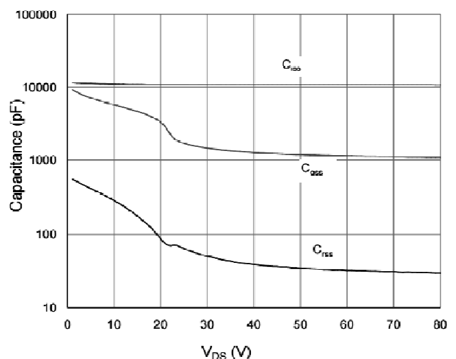
Capacitance
