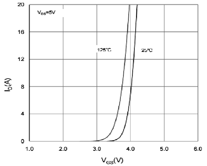
Transfer Characteristic
