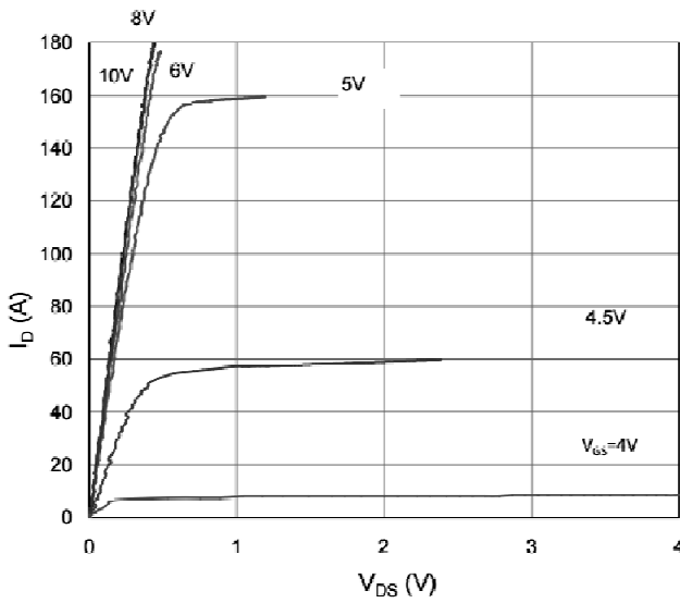
Output Characteristic
